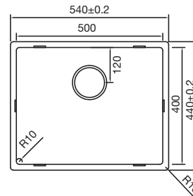
obr. CAPP50R10GM
