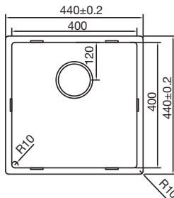
obr. CAPP40R10GM
